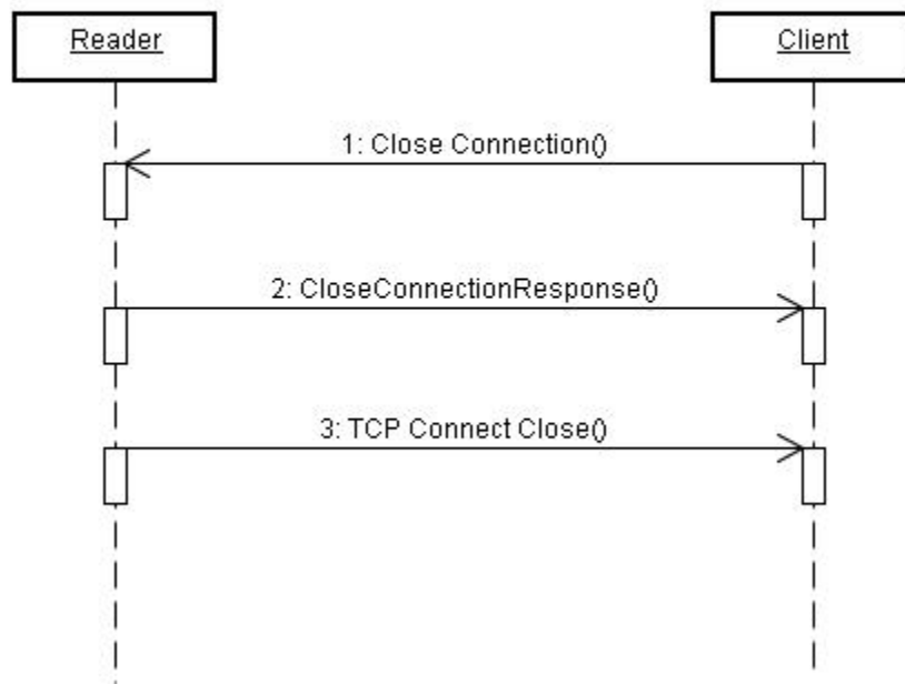
Figure 23: Client Initiated Close (Normal)
