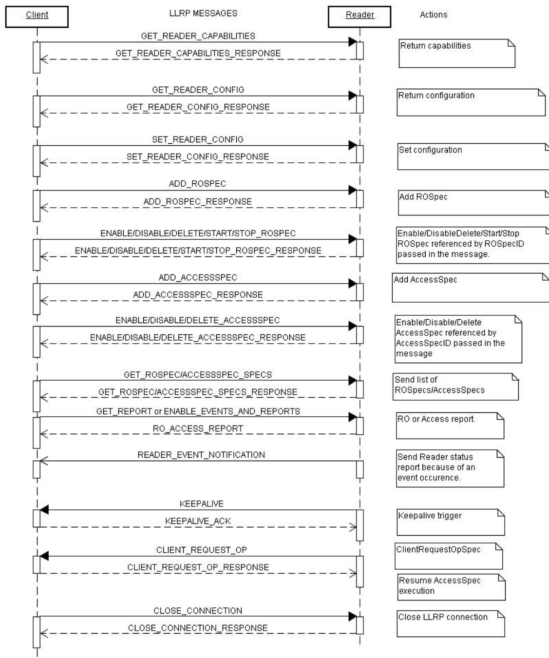
Figure 11: LLRP Messages and Reader Actions
