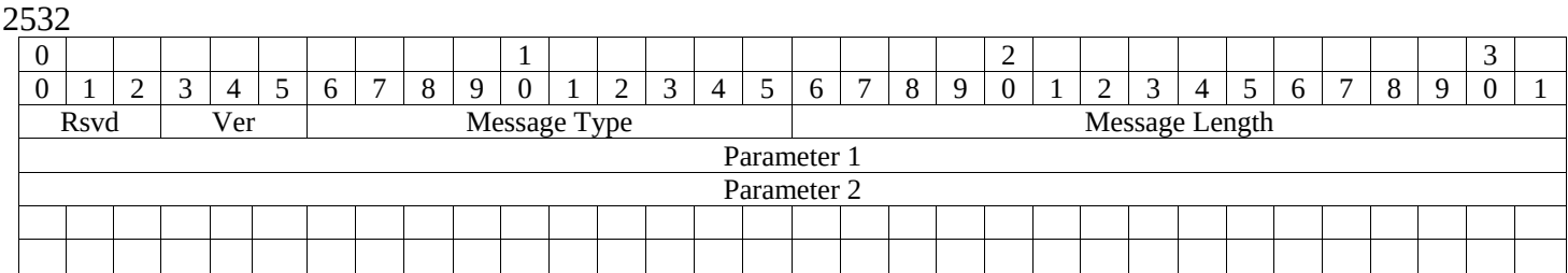
2533 Figure 12: Network Order
