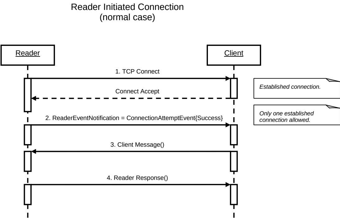
3525 3526 Figure 14: Reader Initiated Connection (Normal) 3527
