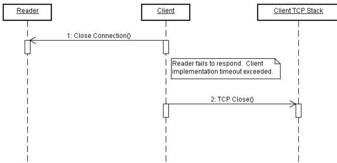
Figure 24: Client Initiated Close (Exception)
