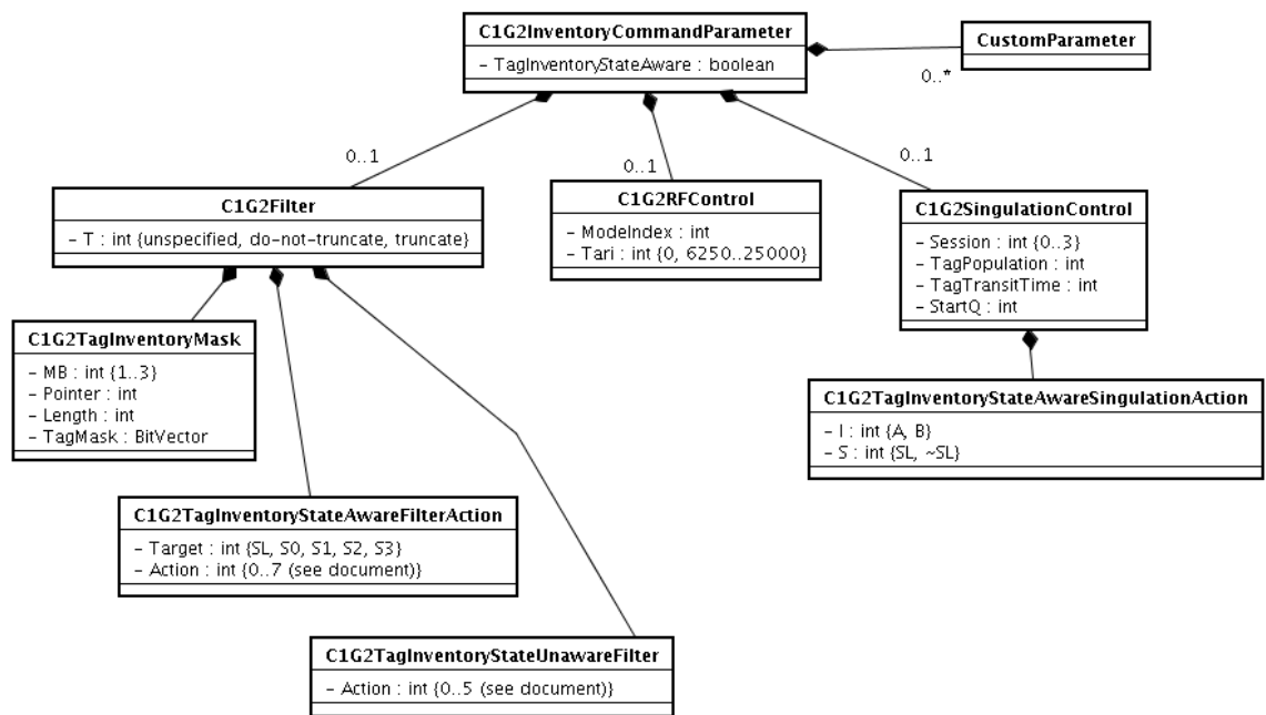
3727 3728 Figure 33: C1G2 Inventory Command
