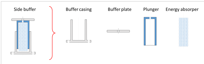
Figure 5-35-3 Side buffer (example of composed MRO-object)
