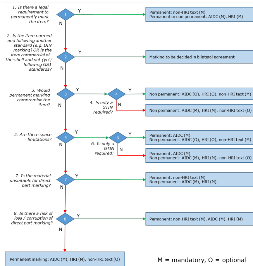
Figure 8-28-2 Direct marking exceptions – decision tree
